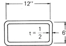
12 X 6 structural tubing A = 15.9 sq in.
