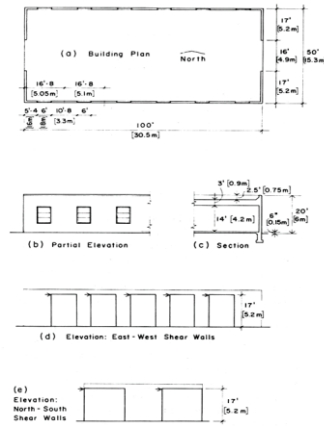
Figure 16.1 Building One, general form.
